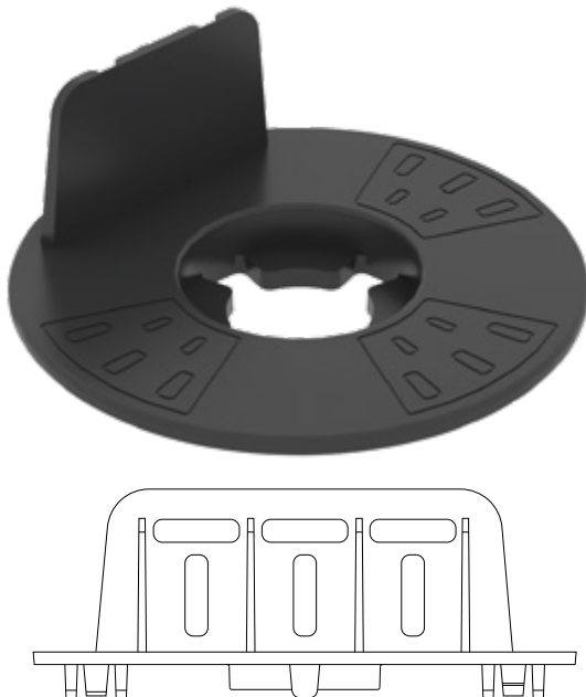
Cabezal Rastrel Madera Wood Batten Head
